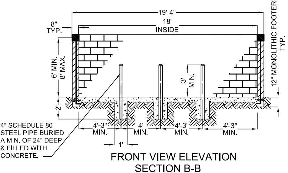
SINGLE DUMPSTER ENCLOSURE WITH RECYCLING AREA
