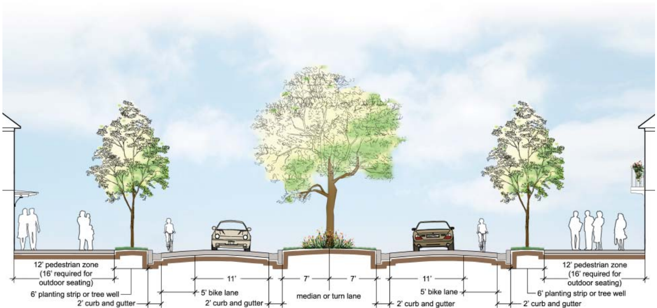
FIGURE 8.3 - CORRIDOR ROAD CROSS SECTION B1/B2 - 2 LANE - 98' Right-Of-Way
