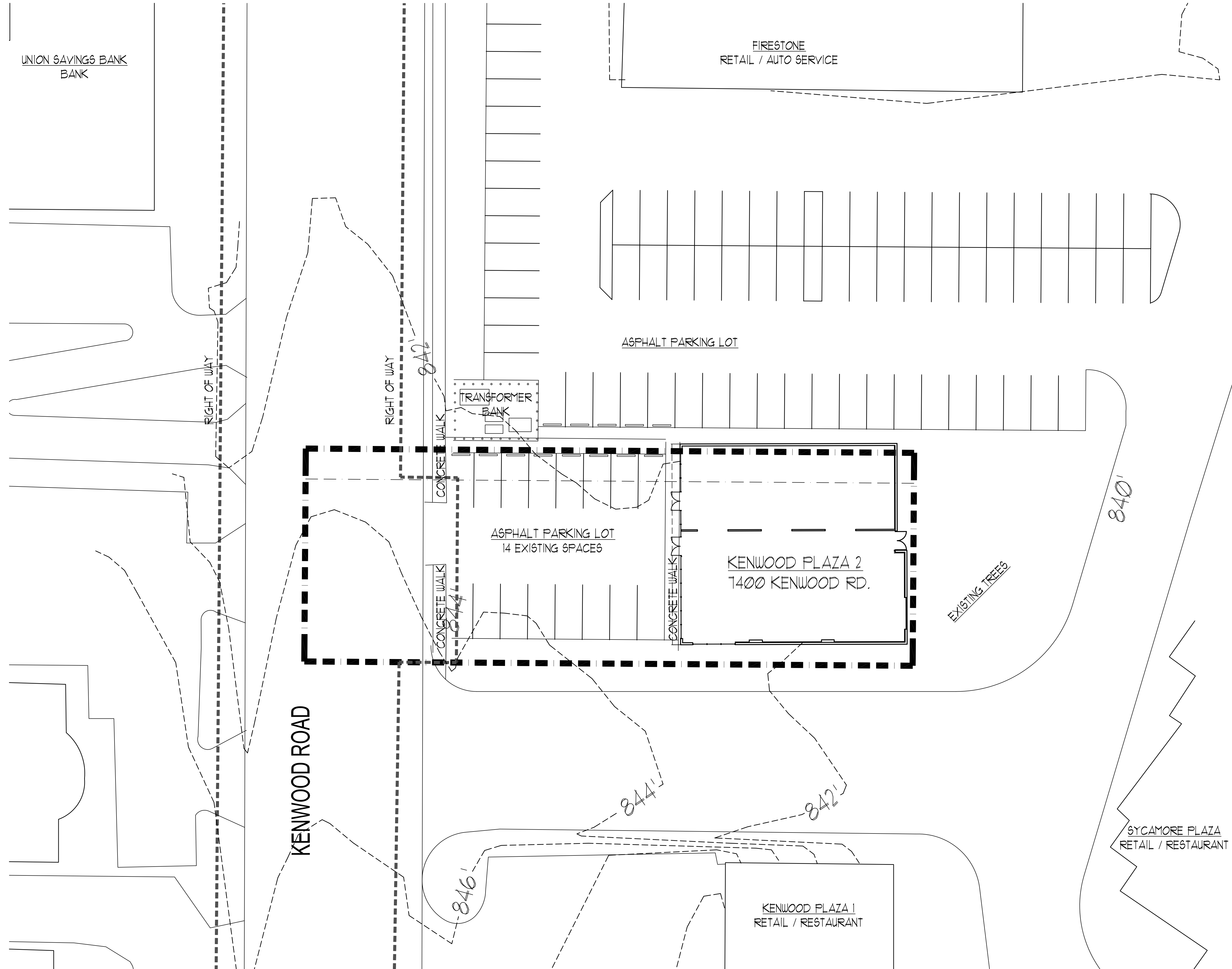
1 EXISTING FEATURES PLAN SCALE: 1/16" = 1'-0"
