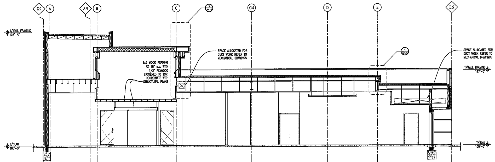
2 BUILDING SECTION SCALE: 3/16" = 1'-0"
