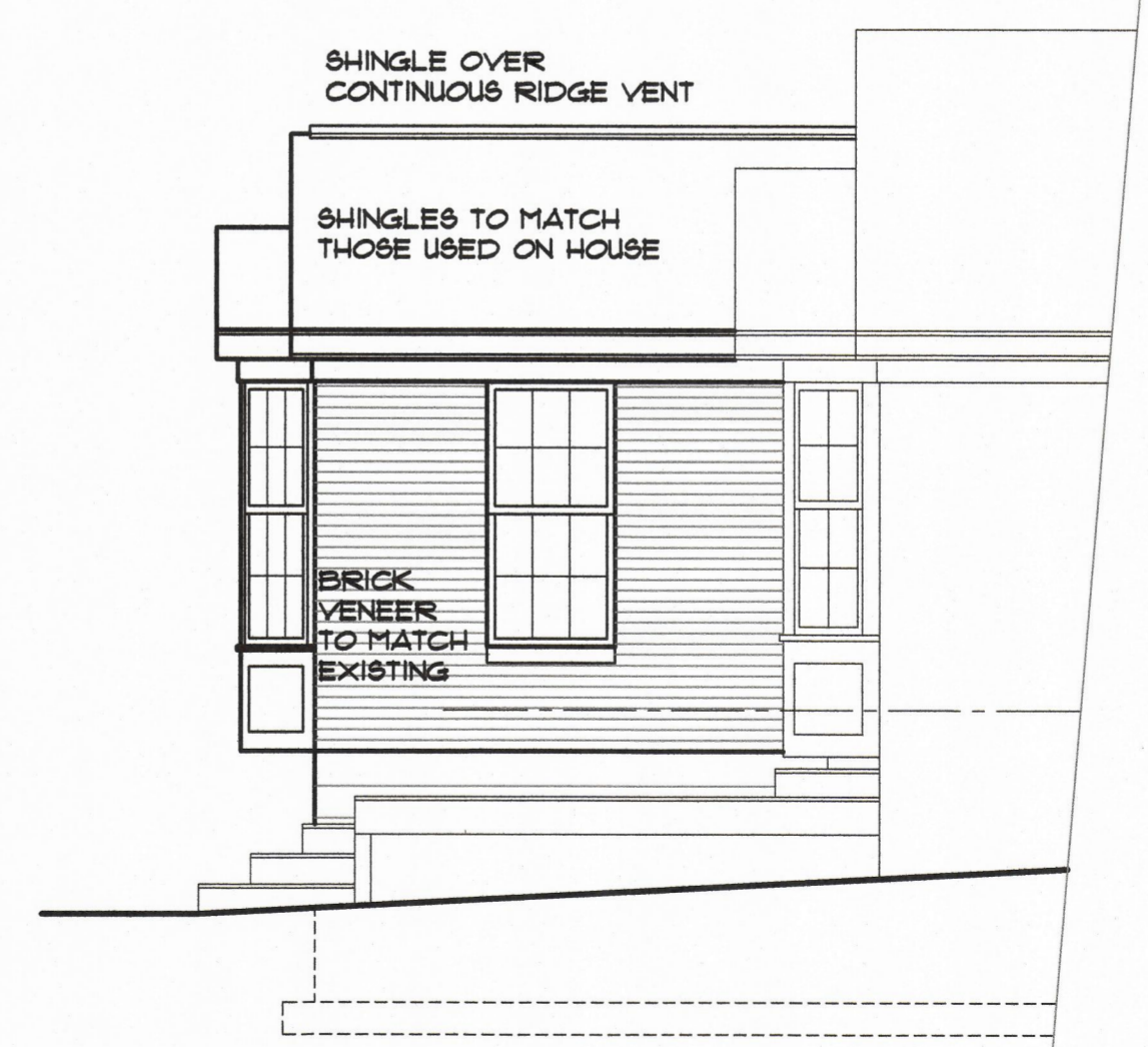
ELEVATION 1/4" = 1'-0" PARTIAL LEFT SIDE
