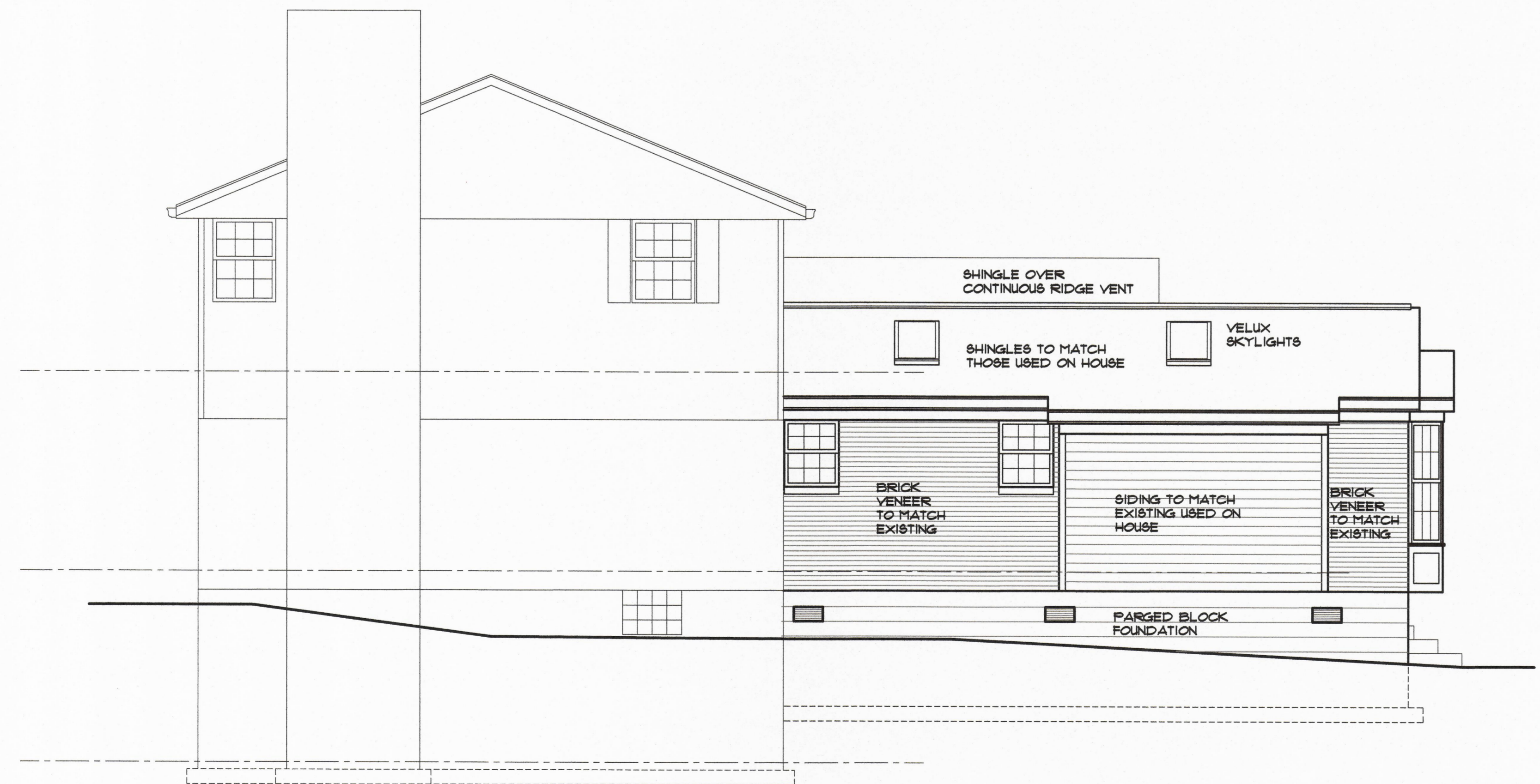
ELEVATION 1/4" = 1'-0" RIGHT SIDE
