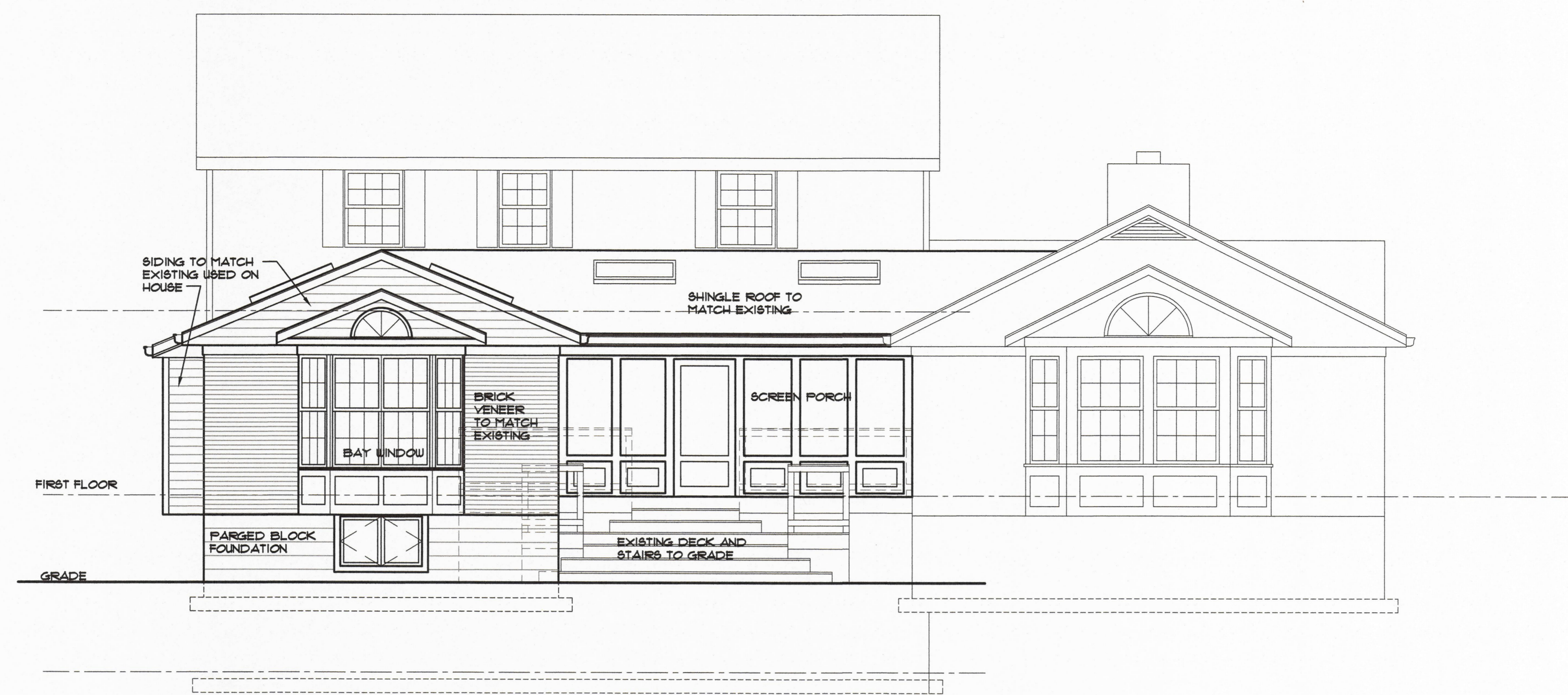
ELEVATION 1/4" = 1'-0" REAR VIEW
