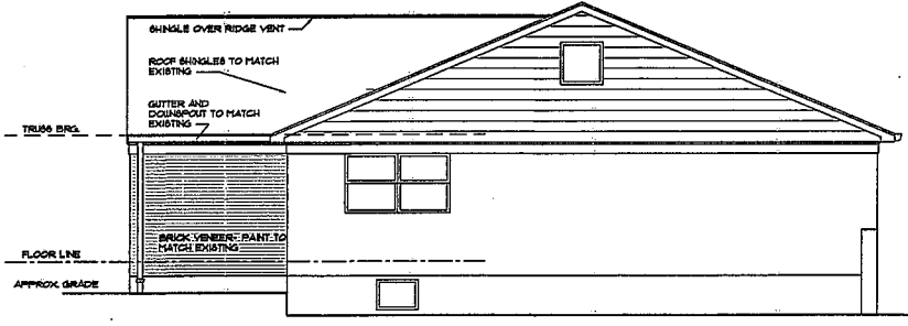
ELEVATION 1/4" = 1'-0" SIDE OF HOUSE
