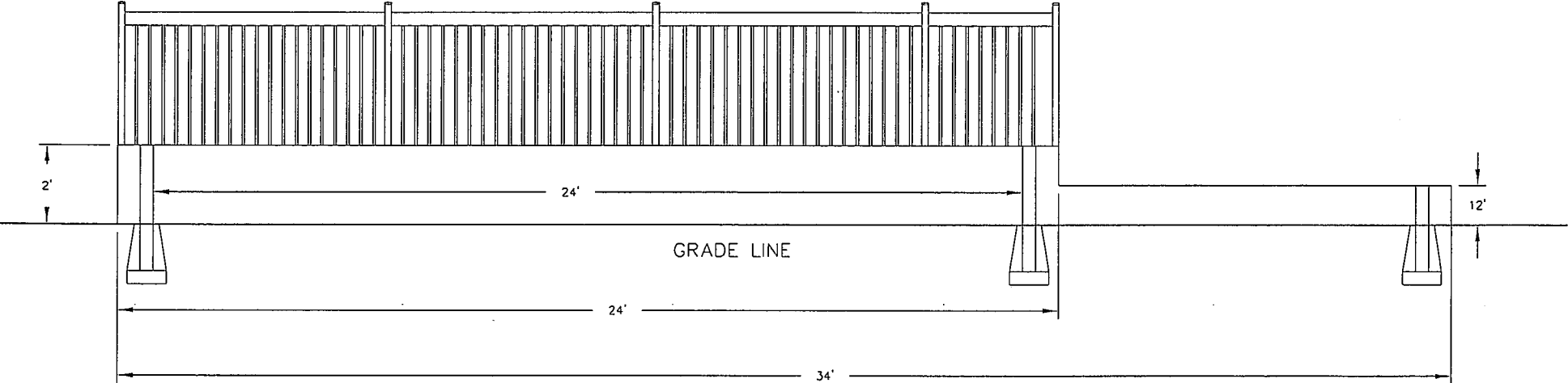
FRONT ELEVATION VIEW
