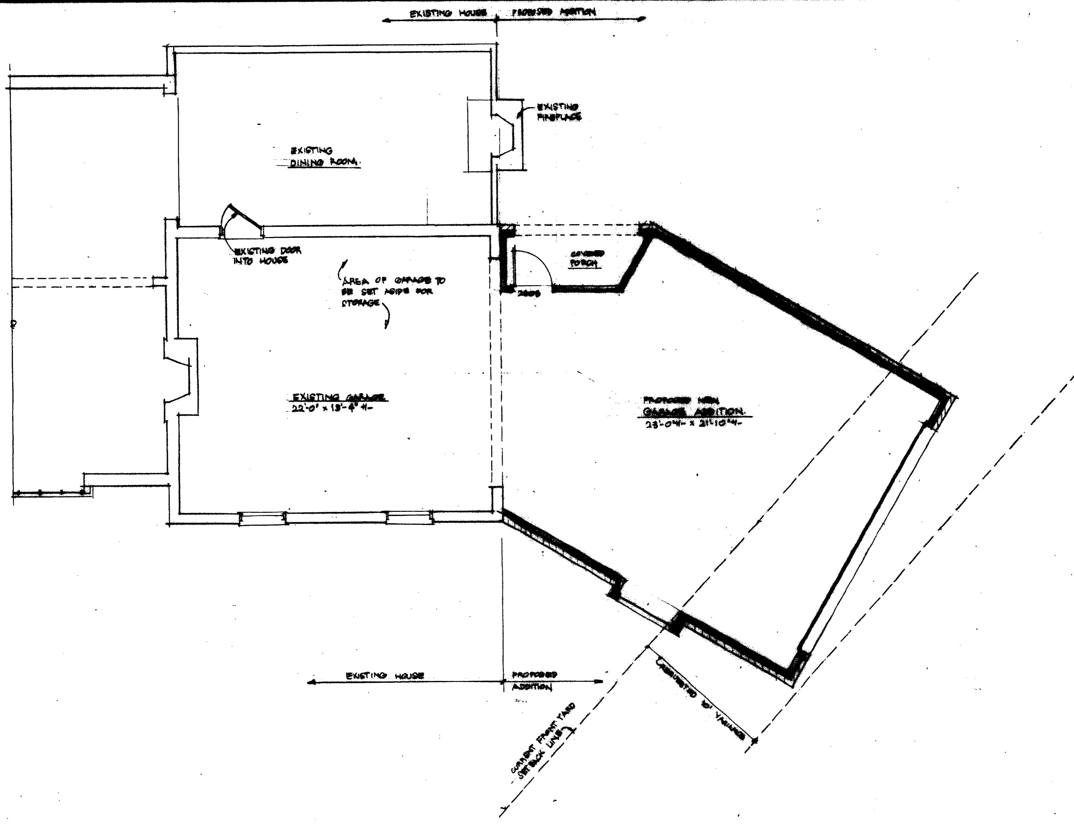
PROPOSED GARAGE ADDITION PLAN
