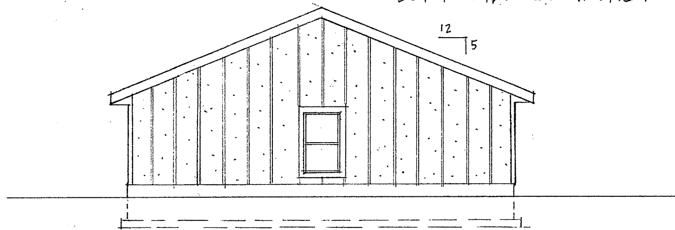
RIGHT-SIDE ELEVATION
