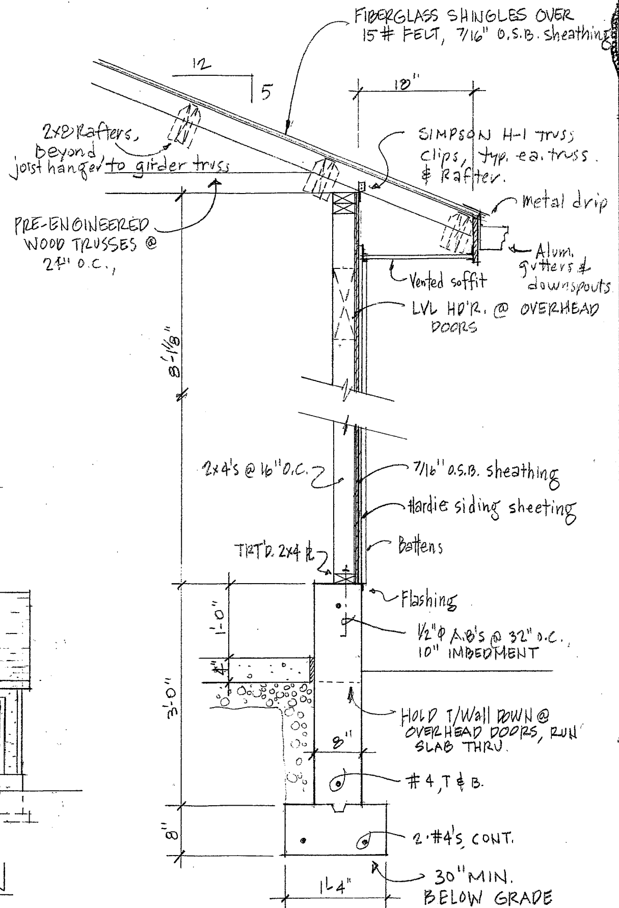
SECTION 3/4" = 1'-0"
