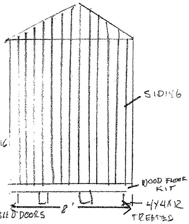
LEFT ELEVATION
