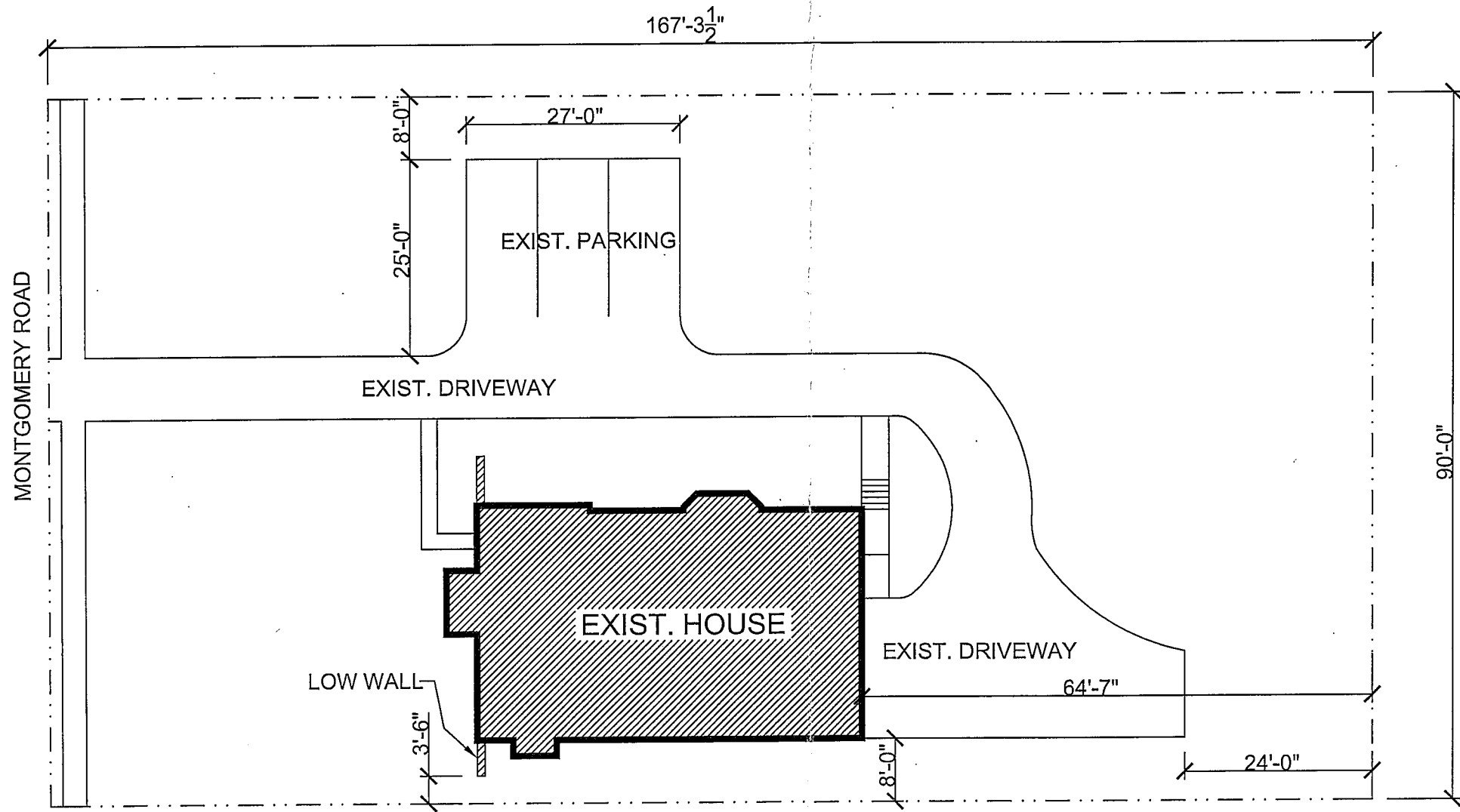
SITE PLAN
