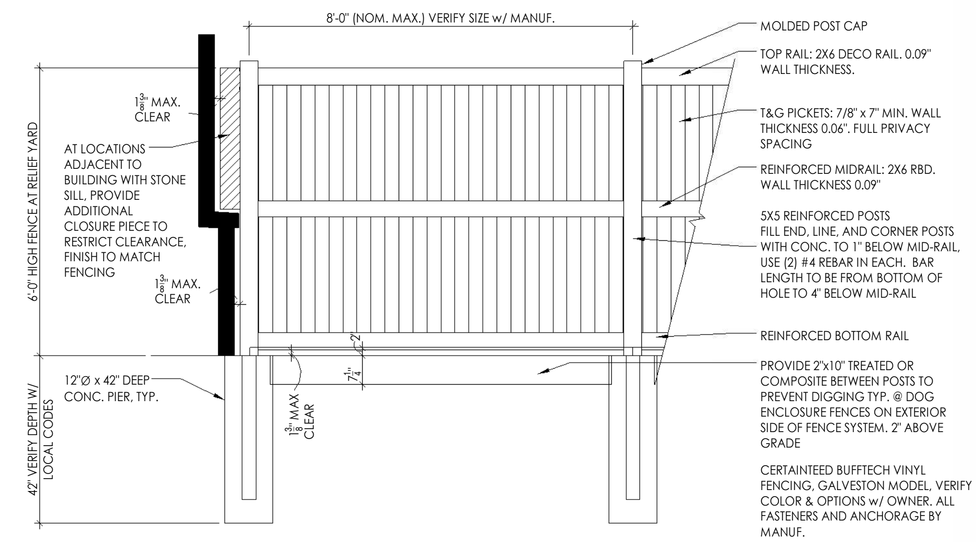
② VINYL FENCE DETAIL 1/2" = 1'-0"
