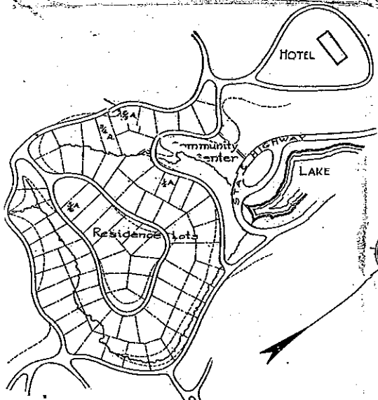
TYPICAL EXAMPLE OF SUBDIVISION ENLARGED SCALE
