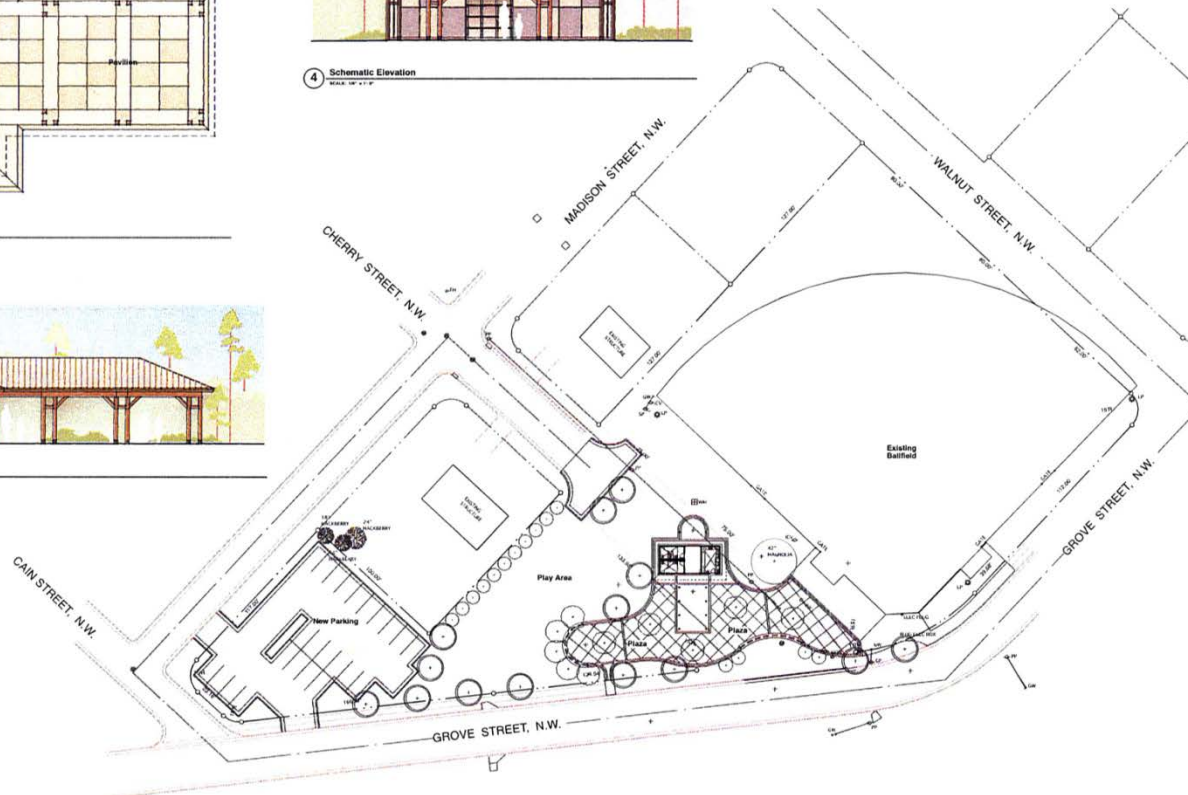
① Site Plan Scale: 1/4" = 1'-0"
