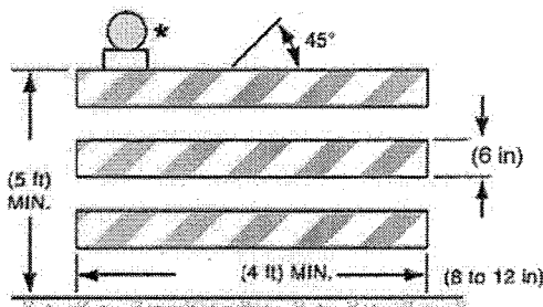
TYPE III BARRICADE with "ROAD CLOSED" sign attached
