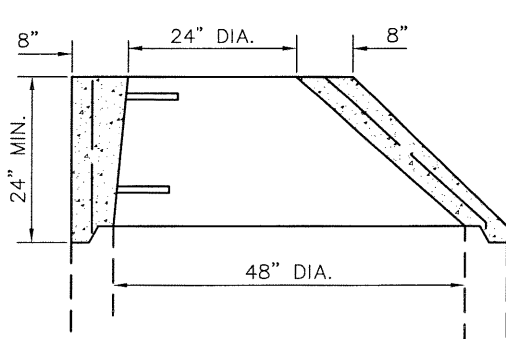
ECCENTRIC CONE TOP
