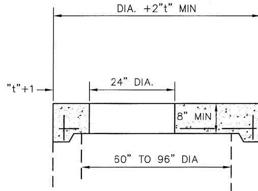
FLAT SLAB TOP
