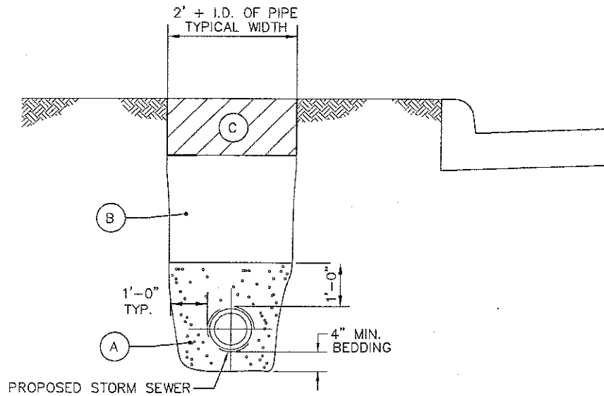
STORM SEWER TRENCH DETAIL (NON-RIGID PIPE)
