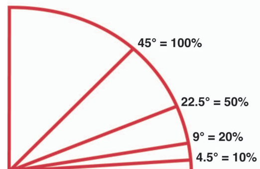
Conversion of Degrees of Angle to Percent Slope
