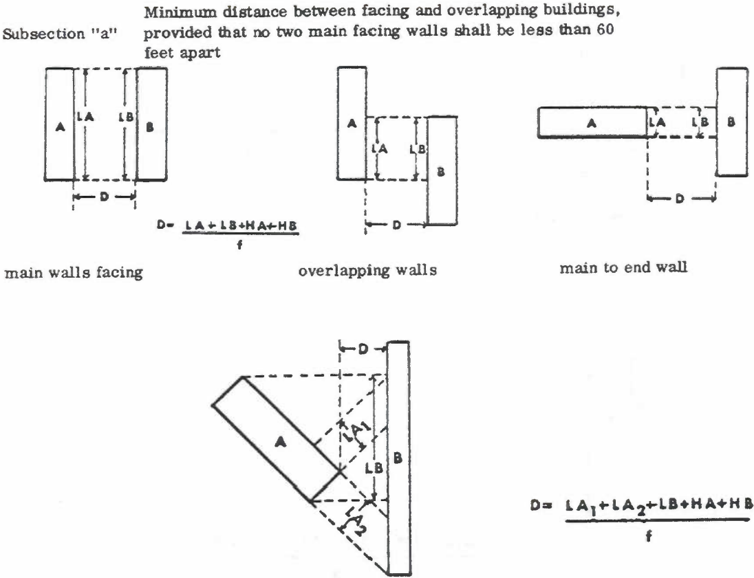
Subsection "b" Minimum distance between oblique facing buildings
