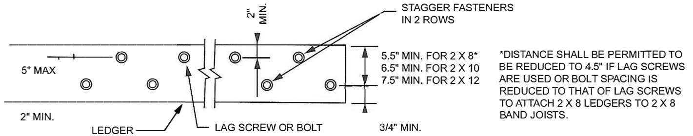
PLACEMENT OF LAG SCREWS AND BOLTS IN LEDGERS
